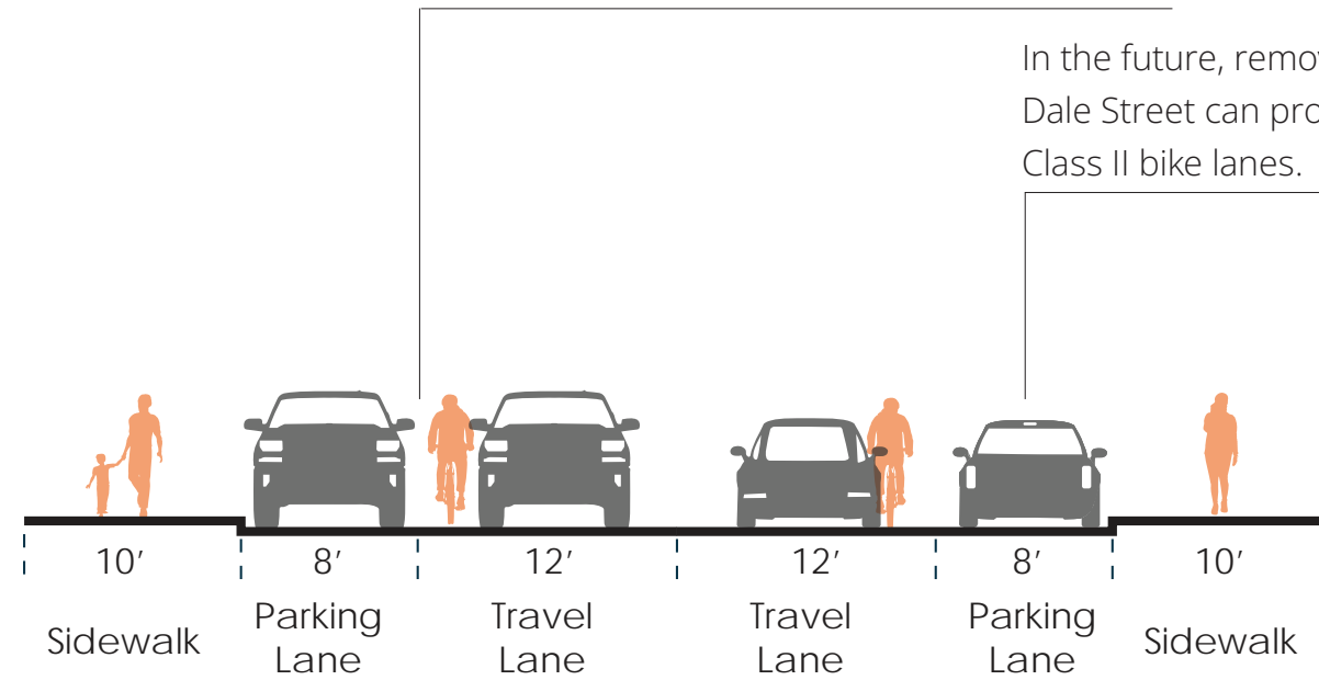
Potential Class IIIb bicycle boulevard in Dale/Augusta Island
