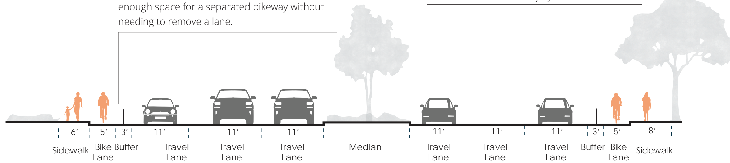
Potential Class IV separated bikeway on Harbor Boulevard in Fountain Valley Island
