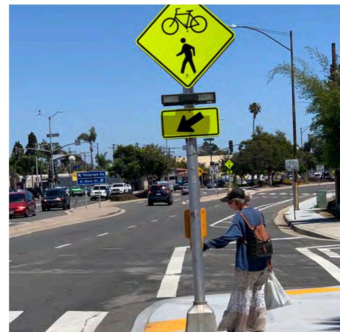
Rapid Rectangular Flashing Beacon (RRFB): when activated by a pedestrian, lights overhead flash alerting drivers that a person is using the crosswalk.
