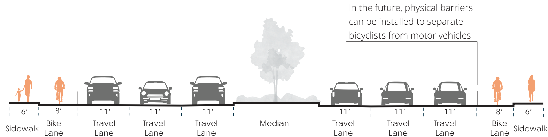
Potential Class IV separated bike lanes on Antonio Parkway in Ladera Ranch, Las Flores, and Rancho Mission Viejo
