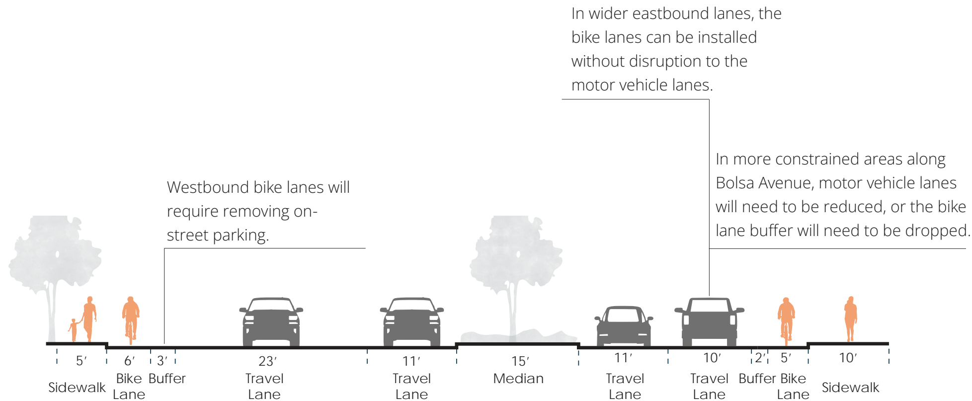
Segment B potential Class IIb buffered bike lanes along Bolsa Avenue between Beach Boulevard and Hunter Lane in Midway City Island
