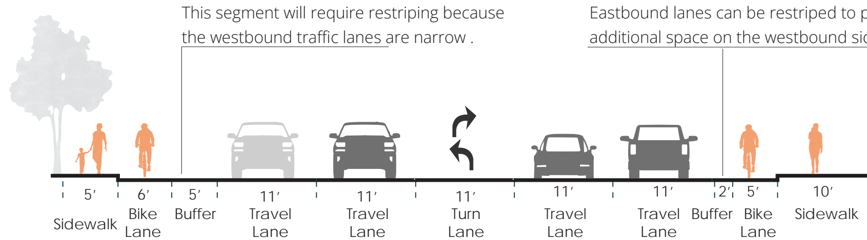
Segment A potential Class IIb buffered bike lanes along Bolsa Avenue between 7750 Bolsa Avenue and Pacific Street in Midway City Island
