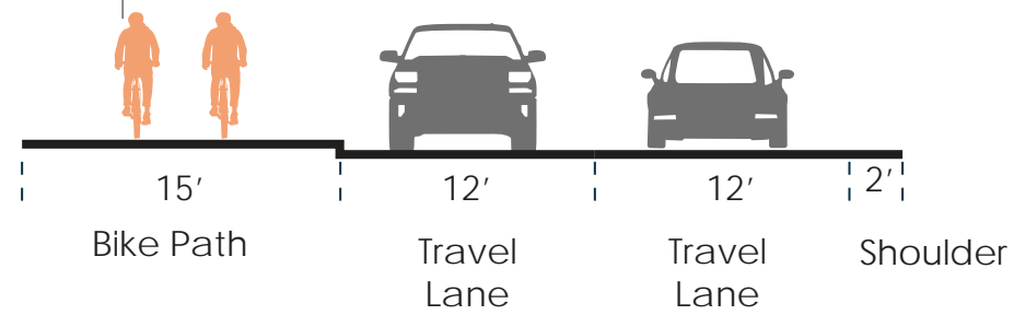
Potential Class I shared-use path along Santiago Canyon Road in Santiago Canyon
