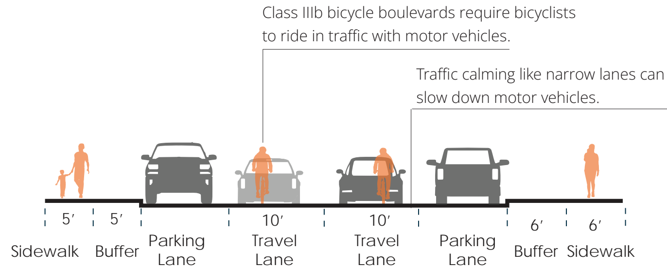
Potential Class IIIb bicycle boulevard along Gilbert Street between just south of Marian Way and Orange Avenue in Anaheim Island
