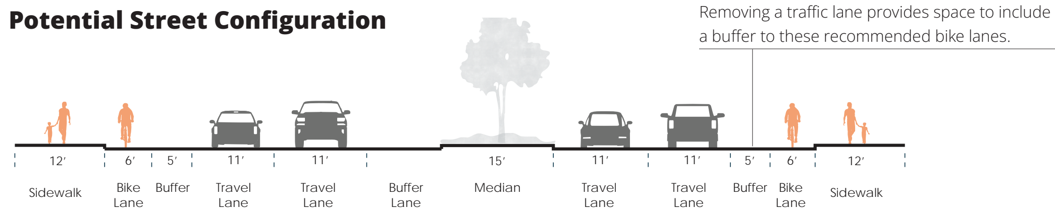
Segment A potential Class II bike lanes along Katella Avenue between Mac Murray Street and Magnolia Street
