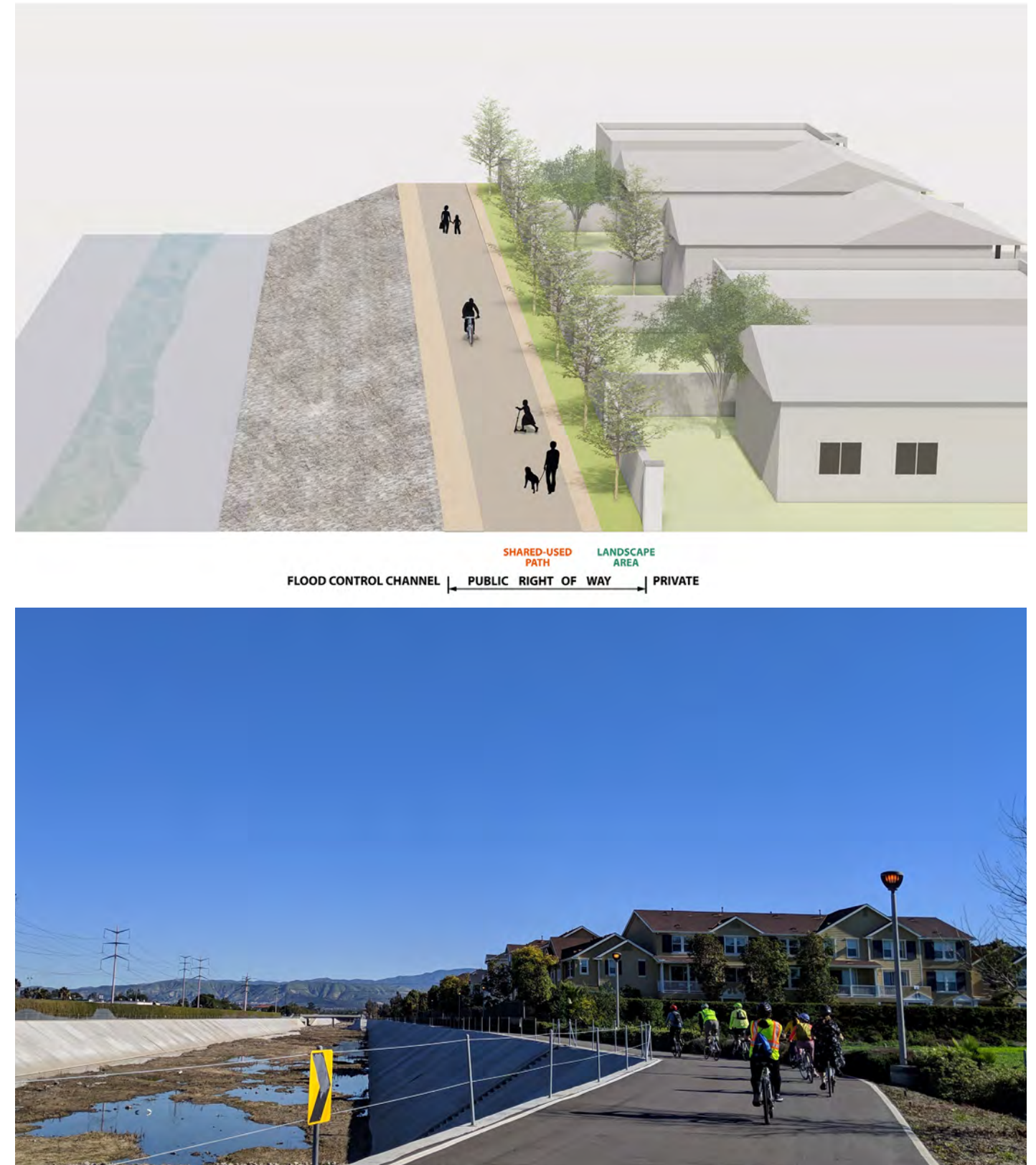
FIGURE 105 Class I: Flood Control
