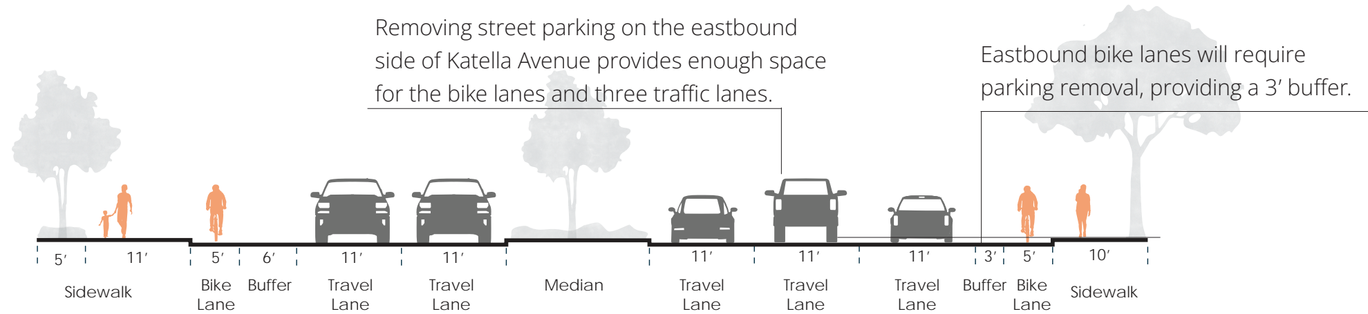
Segment B potential Class II bike lanes along Katella Avenue between Magnolia Street and Rustic Lane
