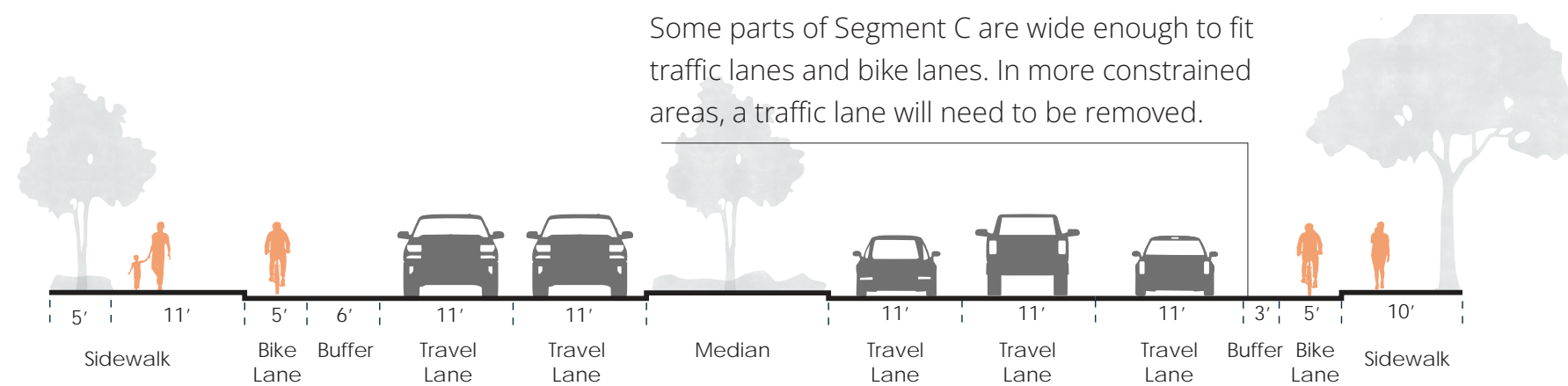
Segment C potential Class II bike lanes along Katella Avenue between Jean Street and Berry Avenue
