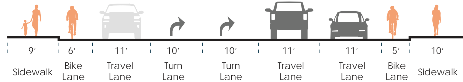
Potential Class II bike lanes with travel lane removal on McFadden Avenue in Midway City Island
