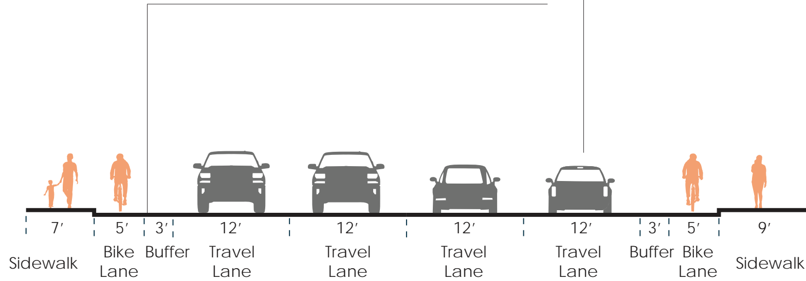
Potential Class II bike lanes along Holt Avenue in North Tustin
