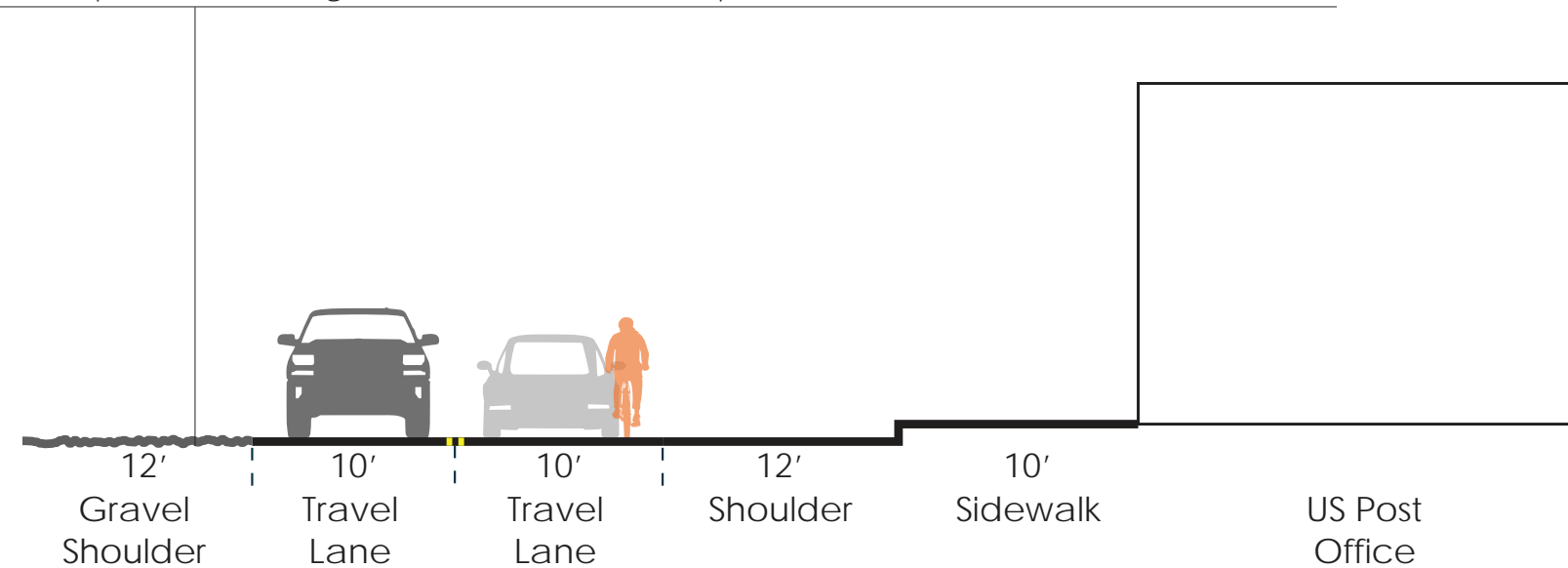
Potential Class IIIb bicycle boulevard in Silverado Canyon near Ladd Canyon Road
