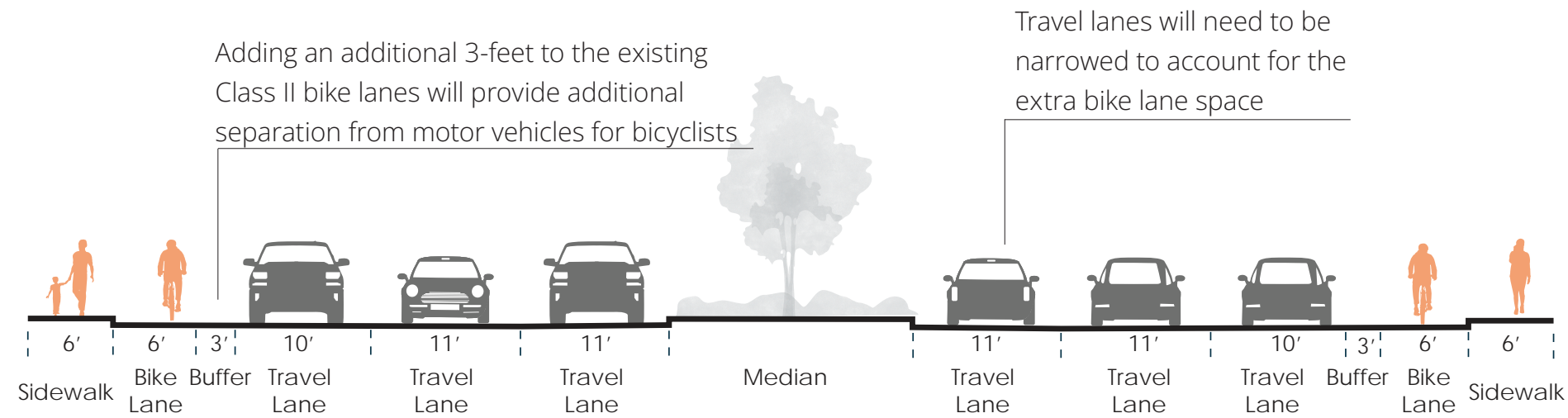
Potential Class IIb buffered bike lanes on Antonio Parkway in Ladera Ranch, Las Flores, and Rancho Mission Viejo
