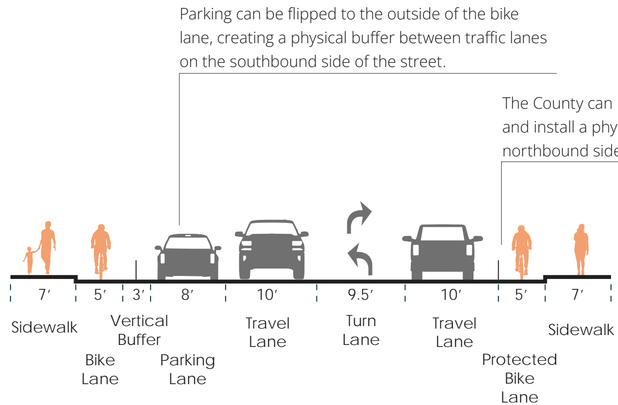
Potential Class IIb buffered bike lanes southbound and potential Class IV separated bikeways northbound along Gilbert Street between Ball Road and Pacific Place in Anaheim Island
